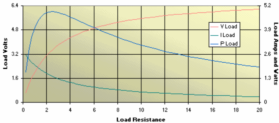
Figure 7: V-I characteristics of a module with a 125 degree temperature differential.
